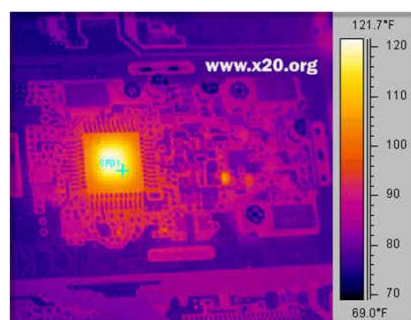
Thermal image of a circuit board
