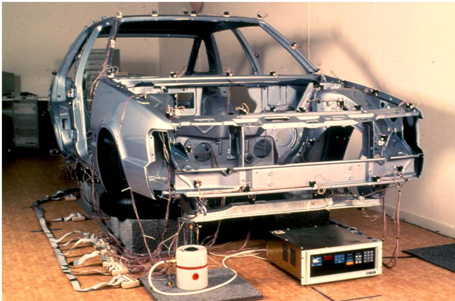
Passenger car modal test
