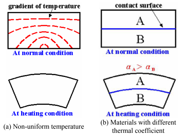
Fig. 6 Two types of thermal deformation
