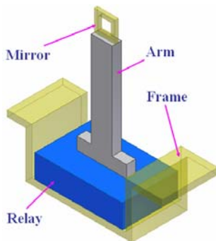
Fig. 9 Structural materials of actuator
