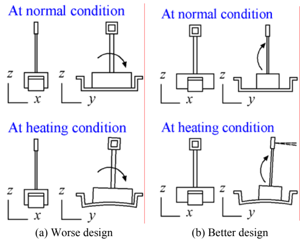
Fig. 10 Two types of holders and mirrors
