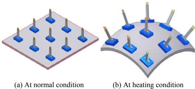
(a) At normal condition (b) At heating condition Fig. 5 The thermal deformation of optical switches
