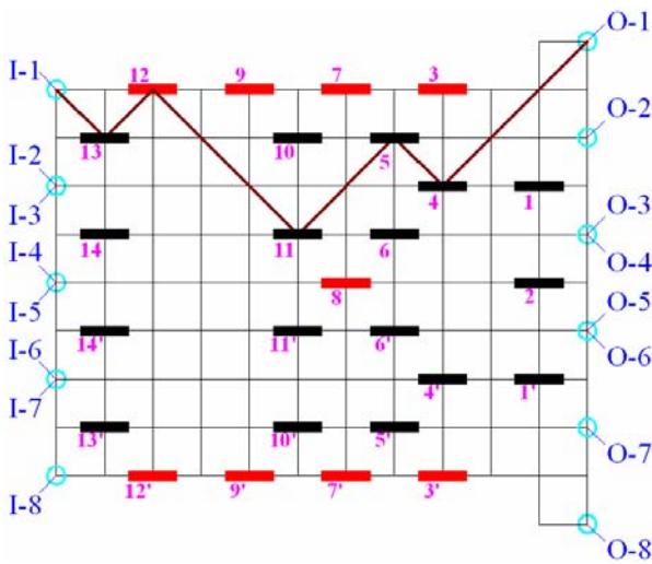
Fig. 16 An optical path with maximum misalignment
