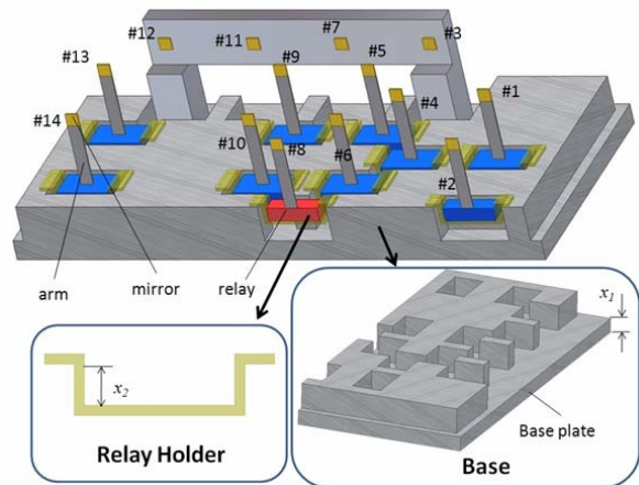
Fig. 17 The geometric structure of 8x8 optical switch
