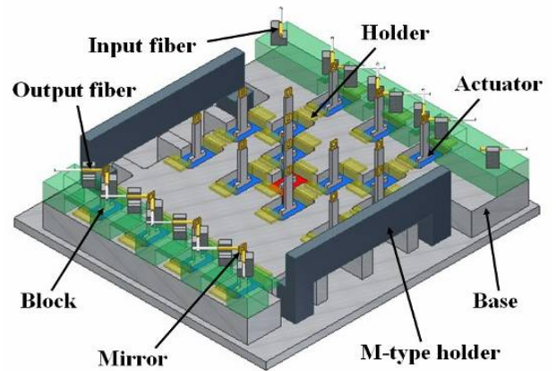
Fig. 3 The model of 8x8 optical switch
