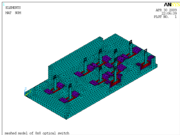
Fig. 12 Meshed model in working condition
