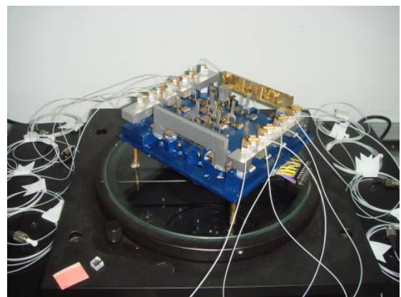
Fig. 4 Prototype of 8x8 optical switch
