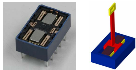
(a) Relay (b) Actuator Fig. 2 The actuator for the optical switch
