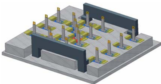
Fig. 8 The structure design for 8x8 optical switch
